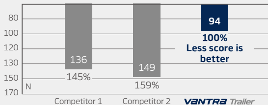
Flat spot (Tire deformation) test result
